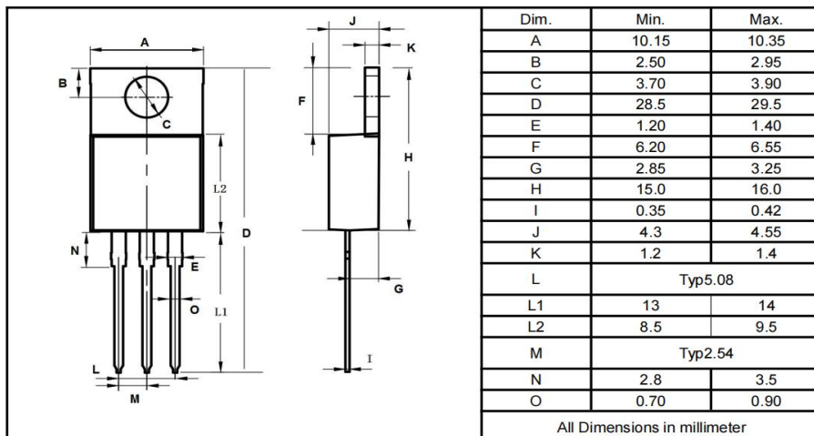
TO-220AB
